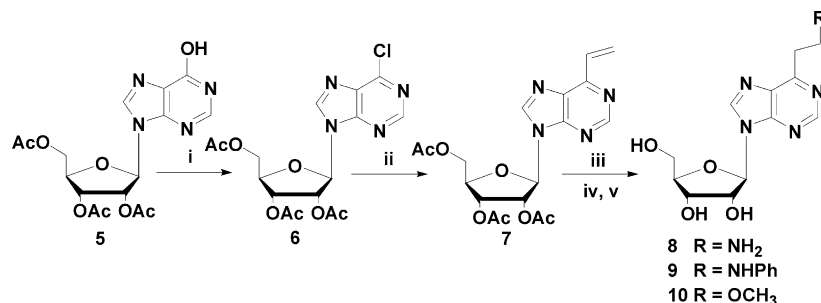
Scheme 2. Regents and conditions: (i) \text{CCl}_4 , HMPT, ACN, 70 °C; (ii) (\text{Ph}_3\text{P})_3\text{PdCl}_2 , tributylvinyltin, DMF, 100 °C; (iii) for compd 8 , \text{NH}_3/\text{CH}_3\text{OH} , rt; (iv) for compd 9 , a. CSA, Aniline, DCM, rt; b. \text{NaOCH}_3/\text{CH}_3\text{OH} , rt; (v) for compd 10 , CSA, \text{NaOCH}_3/\text{CH}_3\text{OH} , rt.
