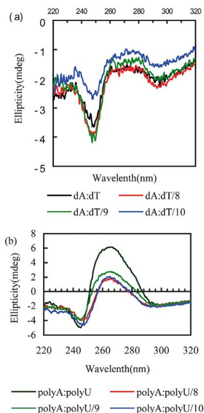
Figure 2. (a) and (b). CD spectra of dA 14 /dT 14 (a) and polyA/polyU (b) in the absence or presence of synthetic 6-substituted 9-β-D-ribofuranosyl purine analogues.
