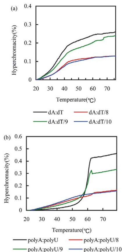
Figure 1. (a) and (b). Thermal melting curves of \text{dA}_{14}/\text{dT}_{14} (a) and polyA/polyU (b) in the absence or presence of synthetic 6-Substituted 9- \beta -D-ribofuranosyl purine analogues.
