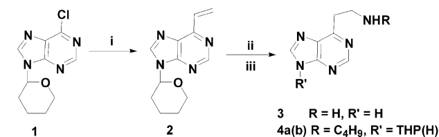
Scheme 1. Regents and conditions: (i) (\text{PhP}_3)_2\text{PdCl}_2 , tributylvinyltin, DCE, reflux; (ii) \text{NH}_3/\text{CH}_3\text{OH} or n\text{-butylamine}/\text{DCM} , rt; (iii) \text{DCM}/\text{CH}_3\text{OH} , 1M HCl, rt.
